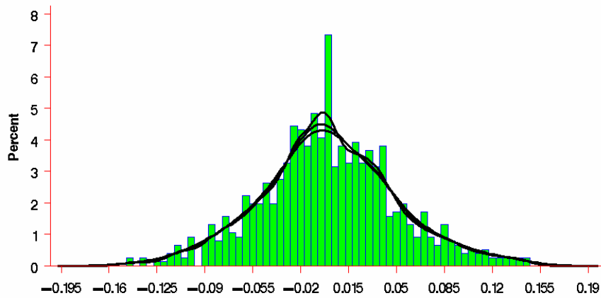
Figure 4. Kernel Density Estimation (Cont.)
